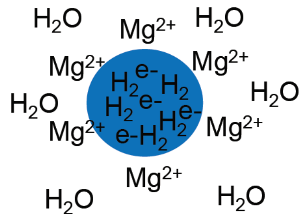
Possible Structure of H 2 Nano-Bubble
